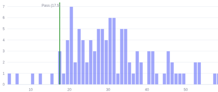
Score Distribution
